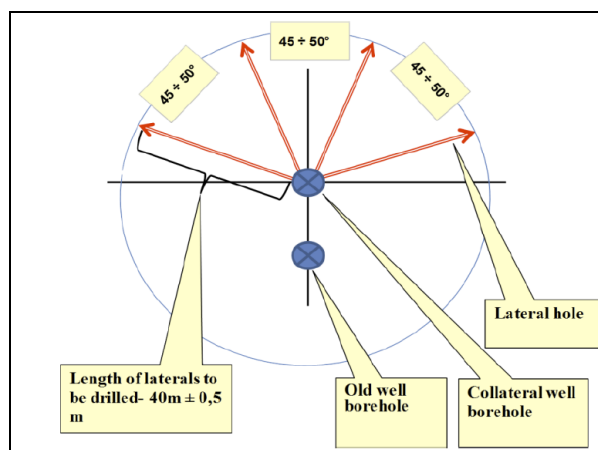
Figure 8: Schematic of laterals to be jetted in Klaipeda Well 1I (Blöcher, et al., 2016).,
