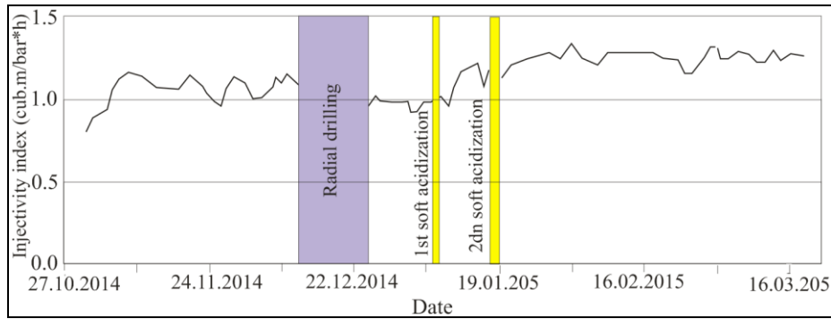
Figure 9: Injectivity index before radial jetting / acidisation and after Klaipeda well 11.
